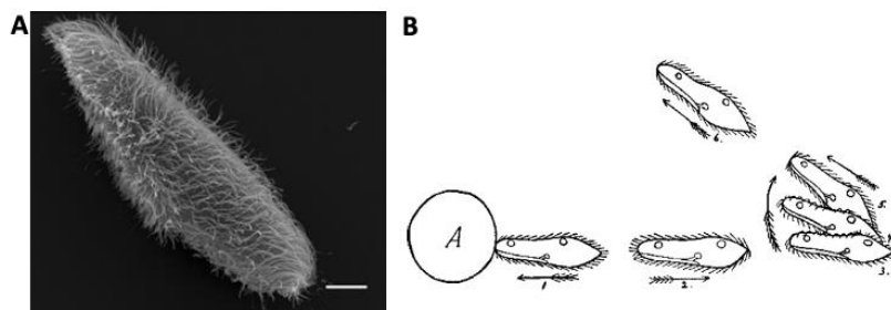
A – Scanning electron microscopy image of Paramecium tetraurelia (scale bar: 10 \mu\text{m} ) (Valentine et al., 2012). B – Avoiding reaction against an obstacle, as illustrated by Jennings (Jennings, 1906).
