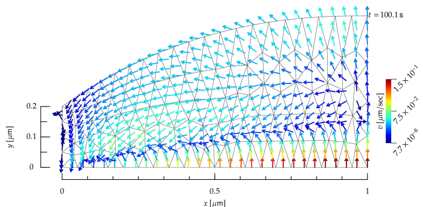
Figure 1: A membrane (curved edge on top) interacting with a bulk fluid, which is in the region where arrows are present. The fluid is injected from the bottom with a velocity directed upwards, and the fluid-velocity direction and intensity is shown by the arrows and color bar, respectively.
